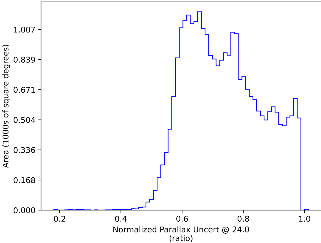
early_u_fpextra2.0_v3.4_10yrs : Normalized Parallax Uncert @ 24.0
