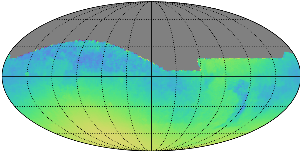
early_u_fpextra2.0_v3.4_10yrs : Normalized Parallax Uncert @ 22.4
