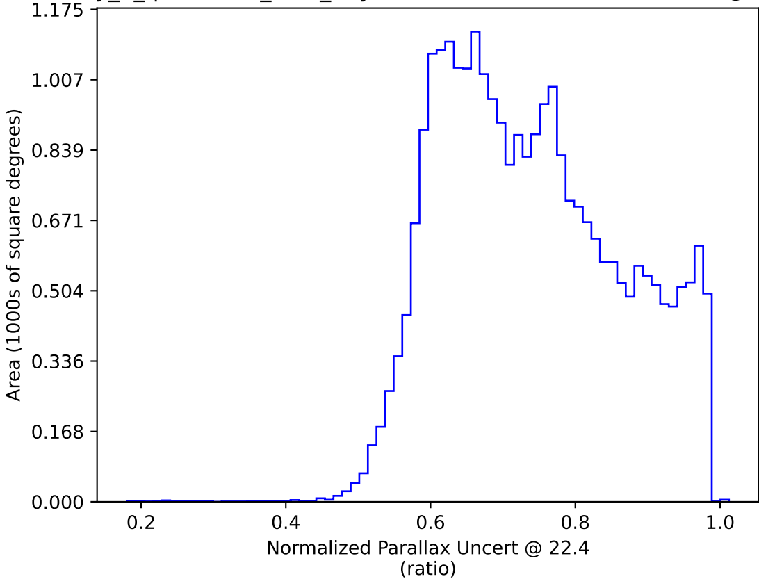
early_u_fpextra2.0_v3.4_10yrs : Normalized Parallax Uncert @ 22.4
