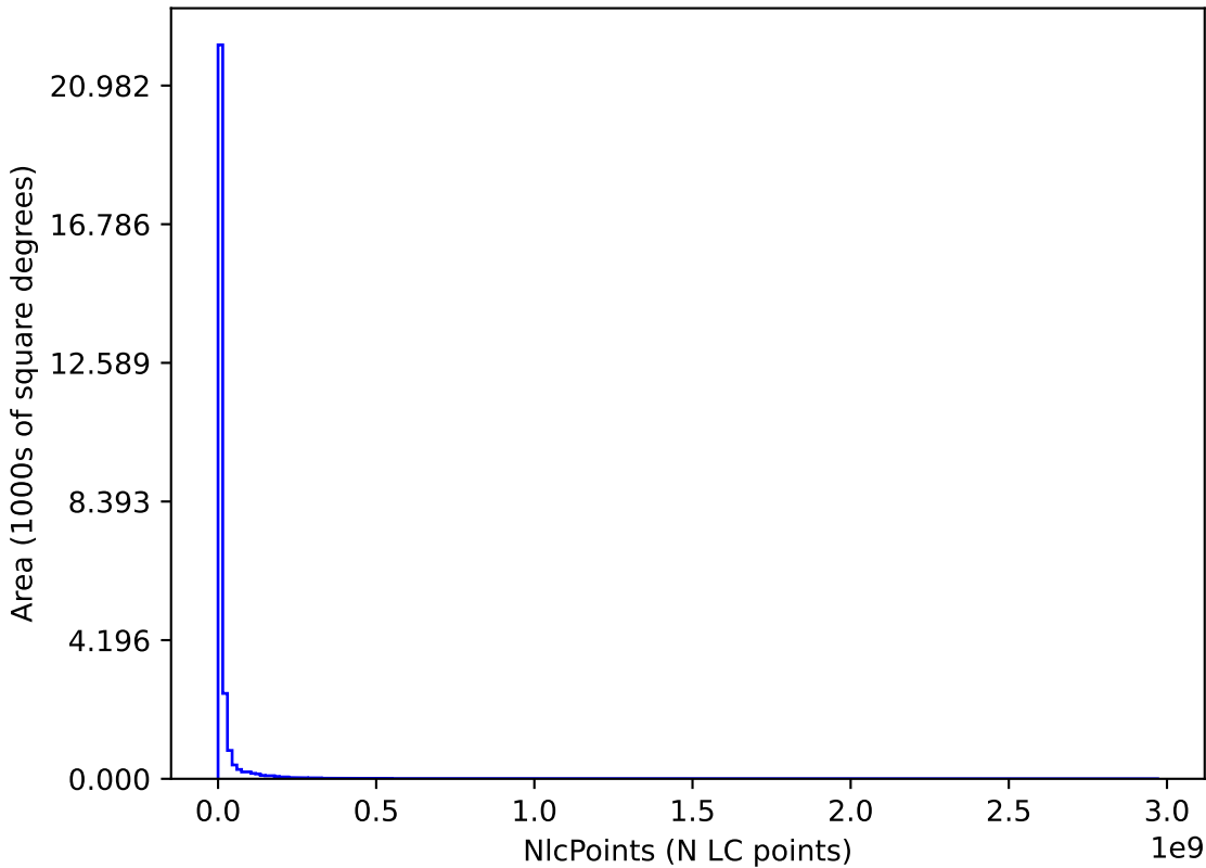
early_u_fpextra2.0_v3.4_10yrs : NlcPoints
