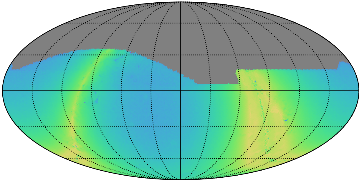
early_u_fpextra2.0_v3.4_10yrs r: N stars to Precision 0.20
