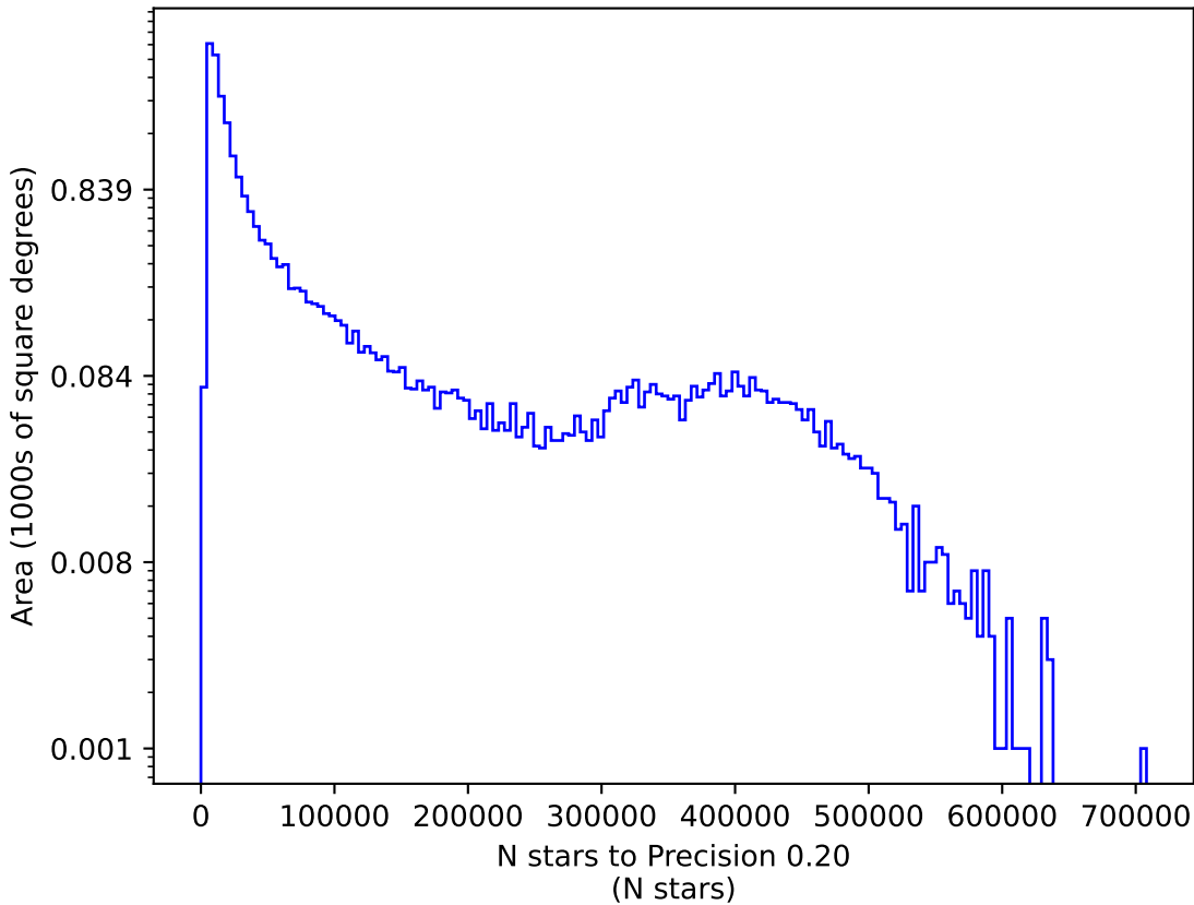
early_u_fpextra2.0_v3.4_10yrs r: N stars to Precision 0.20
