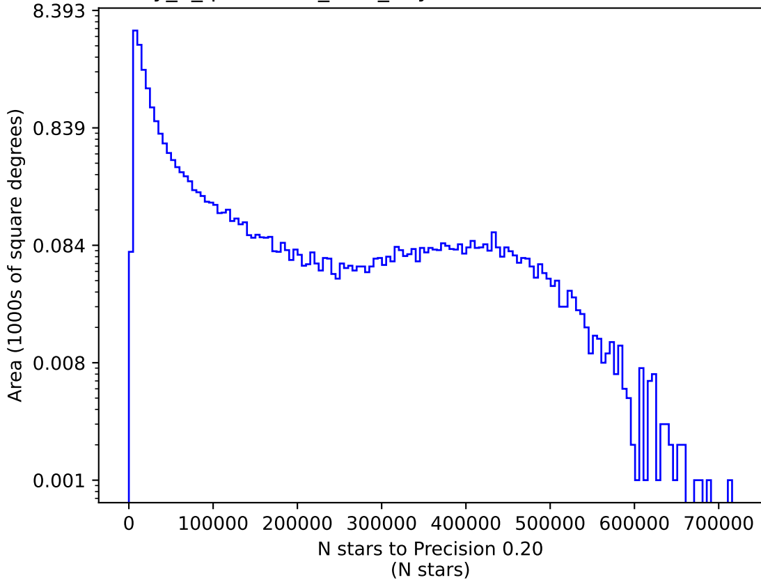
early_u_fpextra2.0_v3.4_10yrs i: N stars to Precision 0.20
