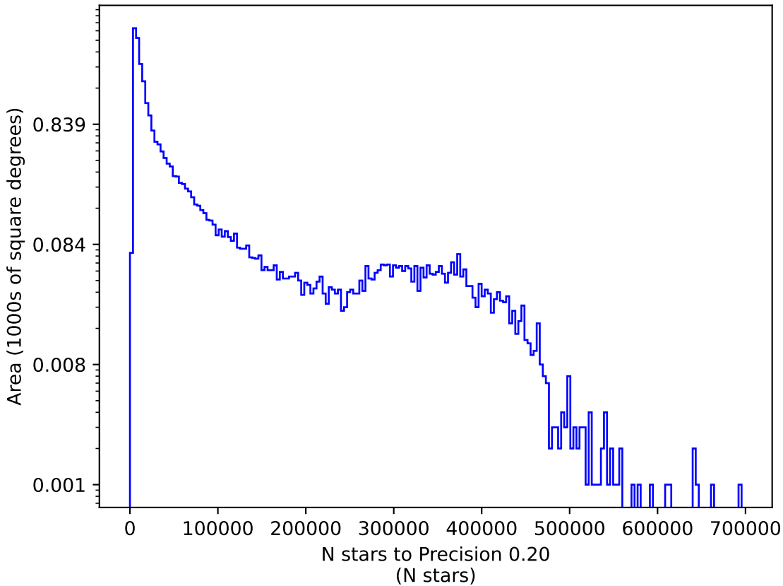
early_u_fpextra2.0_v3.4_10yrs g: N stars to Precision 0.20
