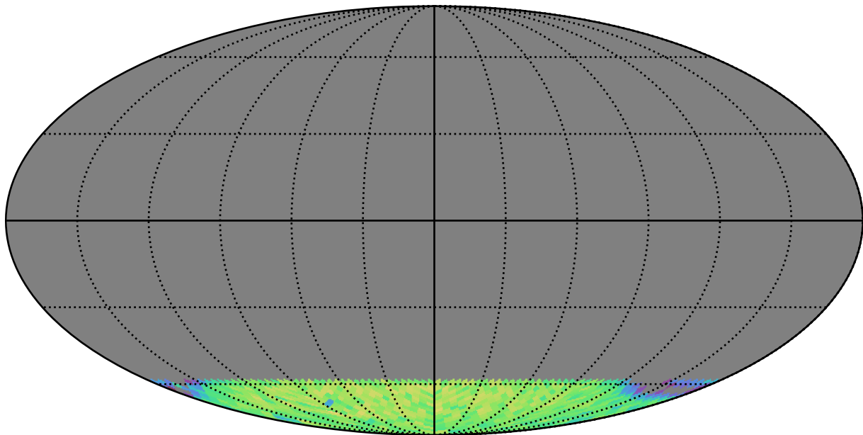
early_u_fpextra2.0_v3.4_10yrs gi SCP: LVDwarfs
