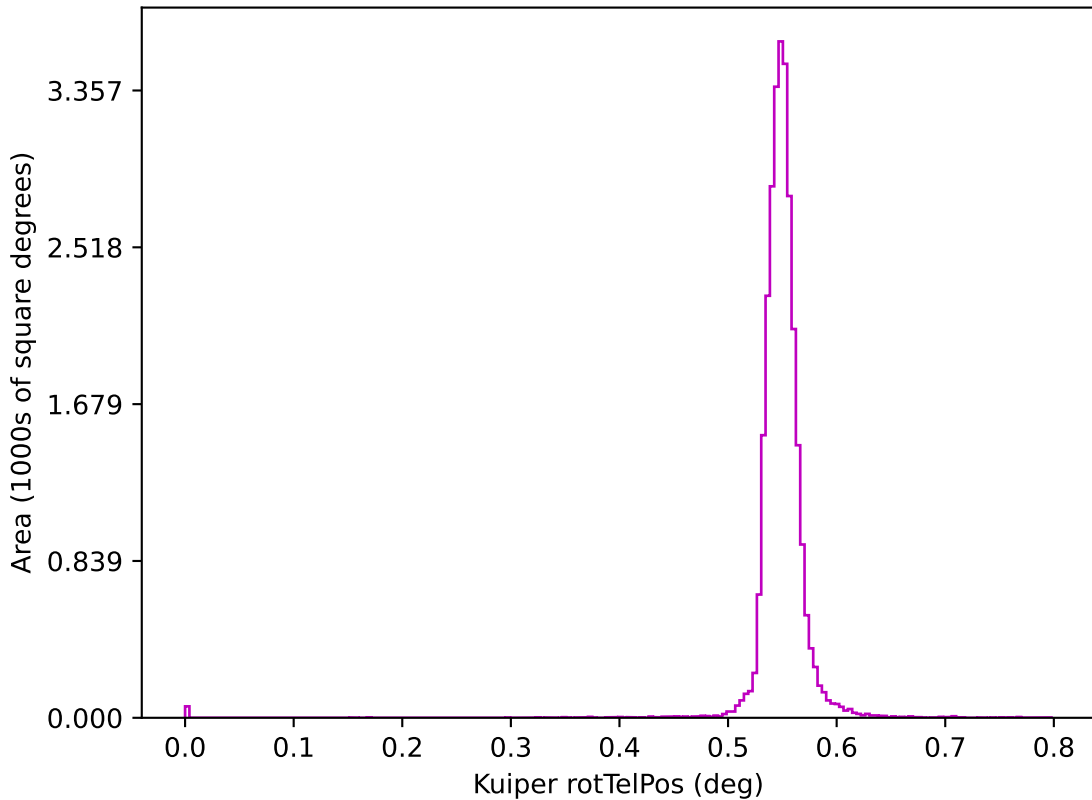
early_u_fpextra2.0_v3.4_10yrs z: Kuiper rotTelPos
