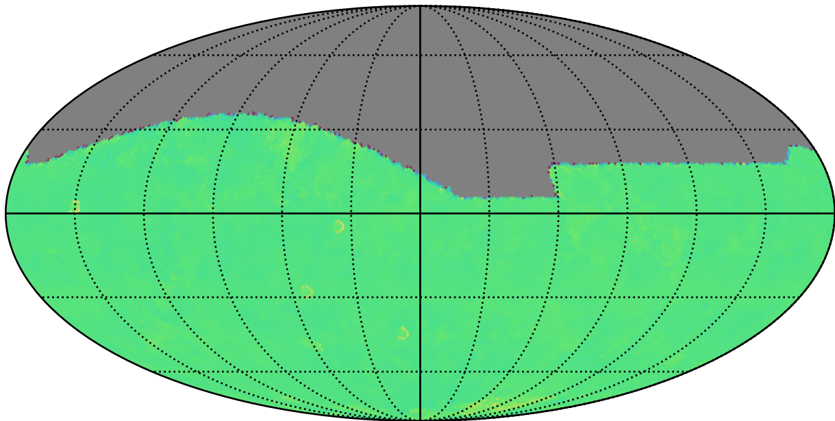
early_u_fpextra2.0_v3.4_10yrs r: Kuiper rotTelPos
