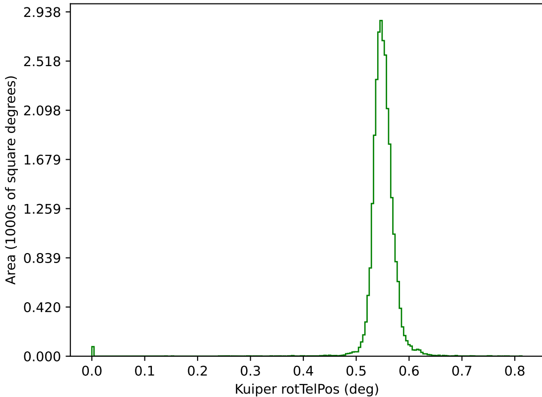
early_u_fpextra2.0_v3.4_10yrs g: Kuiper rotTelPos
