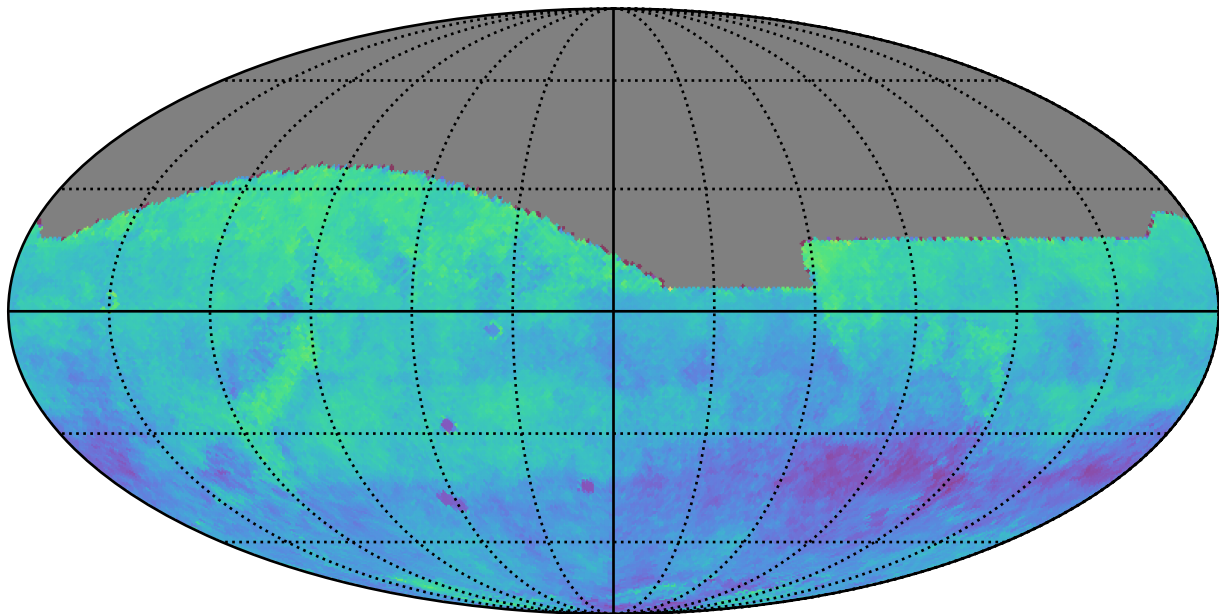
early_u_fpextra2.0_v3.4_10yrs z: Kuiper rotSkyPos
