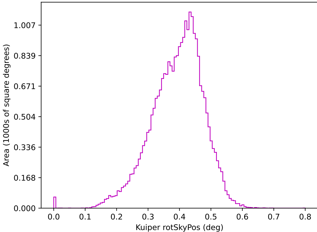
early_u_fpextra2.0_v3.4_10yrs z: Kuiper rotSkyPos
