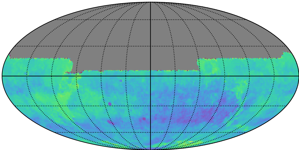
early_u_fpextra2.0_v3.4_10yrs y: Kuiper rotSkyPos
