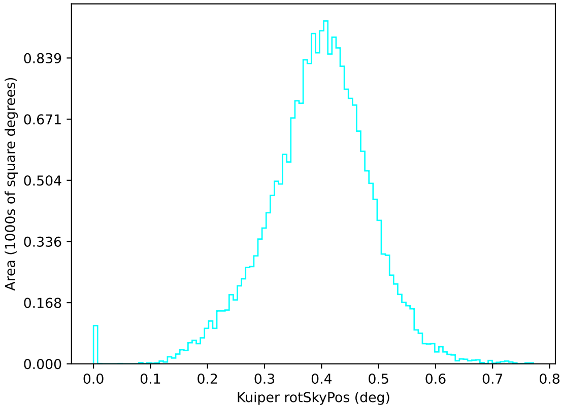
early_u_fpextra2.0_v3.4_10yrs u: Kuiper rotSkyPos
