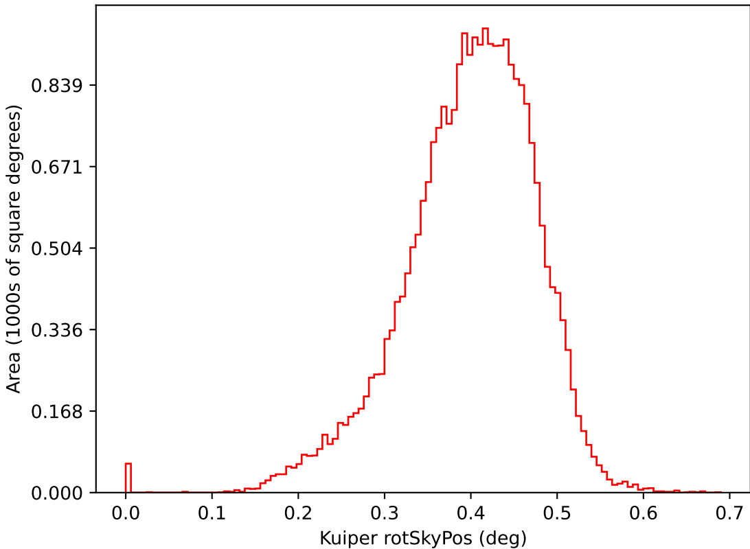
early_u_fpextra2.0_v3.4_10yrs i: Kuiper rotSkyPos
