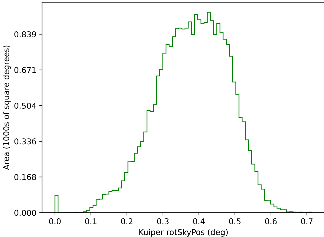
early_u_fpextra2.0_v3.4_10yrs g: Kuiper rotSkyPos
