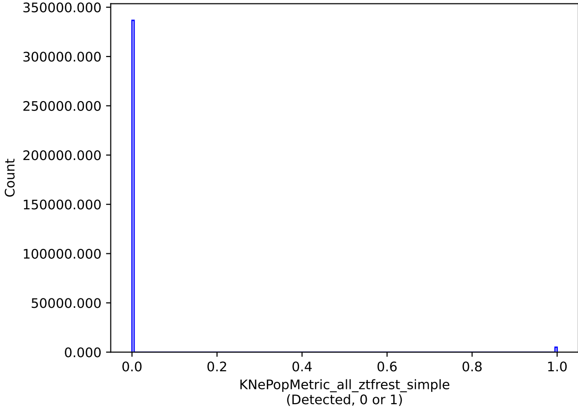
early_u_fpextra2.0_v3.4_10yrs all models: KNePopMetric_all_ztfrest_simple
