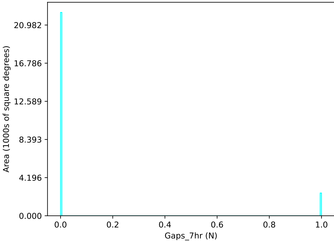
early_u_fpextra2.0_v3.4_10yrs u band: Gaps_7hr
