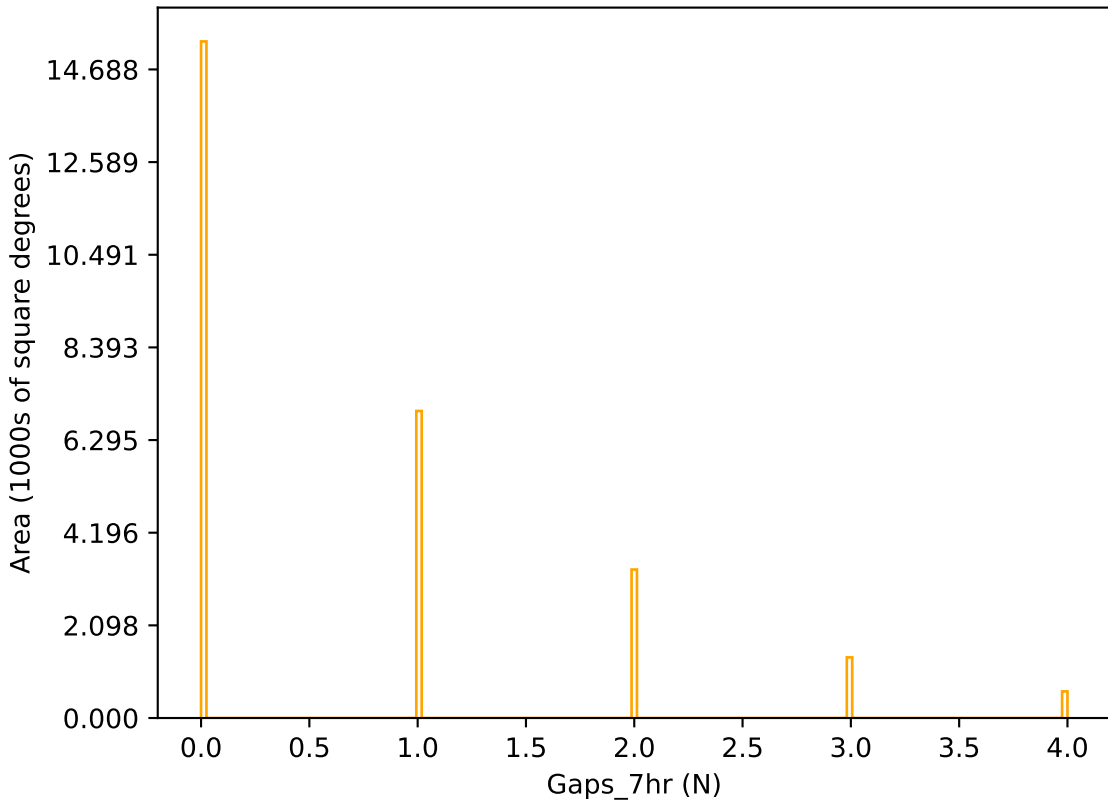
early_u_fpextra2.0_v3.4_10yrs r band: Gaps_7hr
