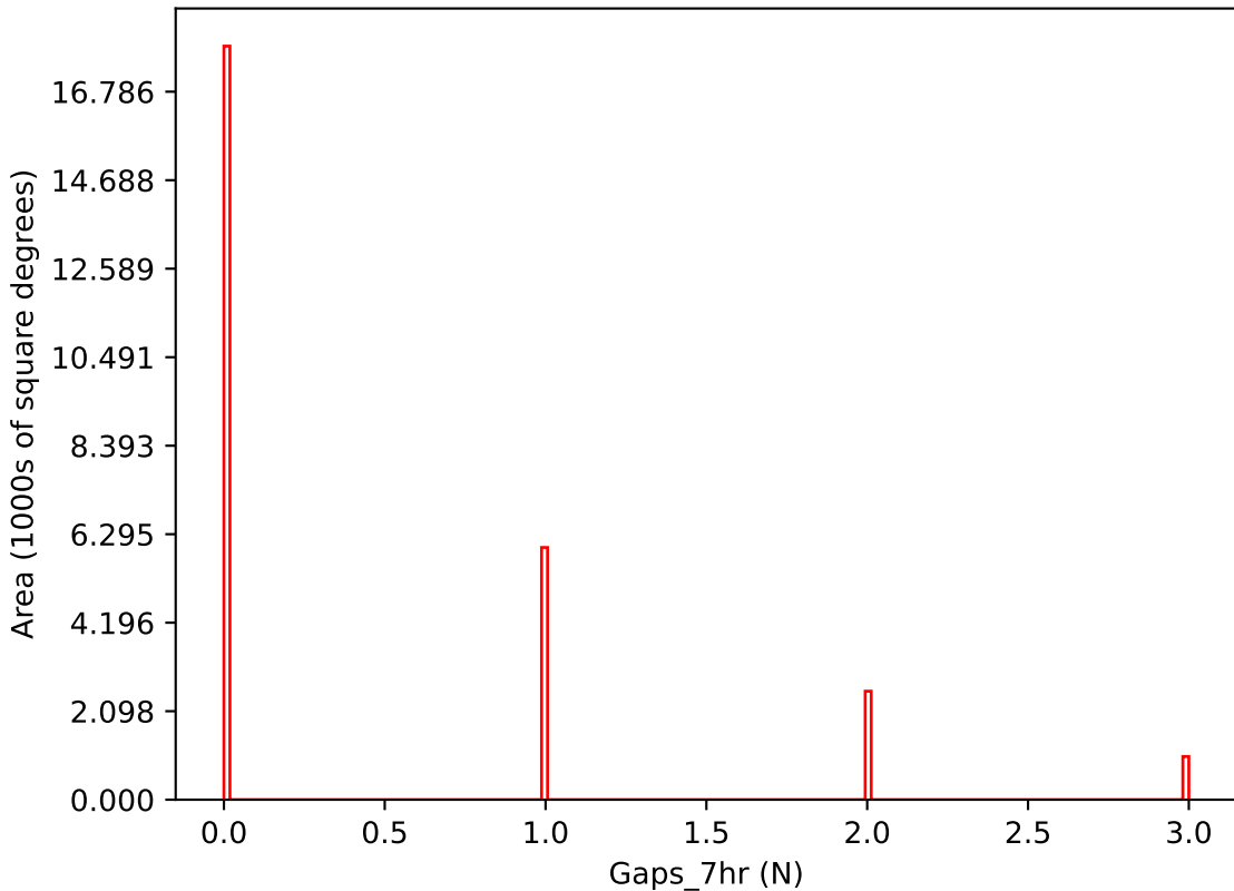
early_u_fpextra2.0_v3.4_10yrs i band: Gaps_7hr
