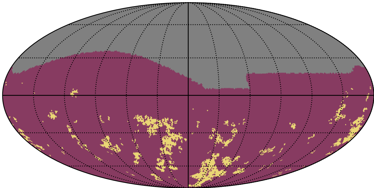
early_u_fpextra2.0_v3.4_10yrs g band: Gaps_7hr
