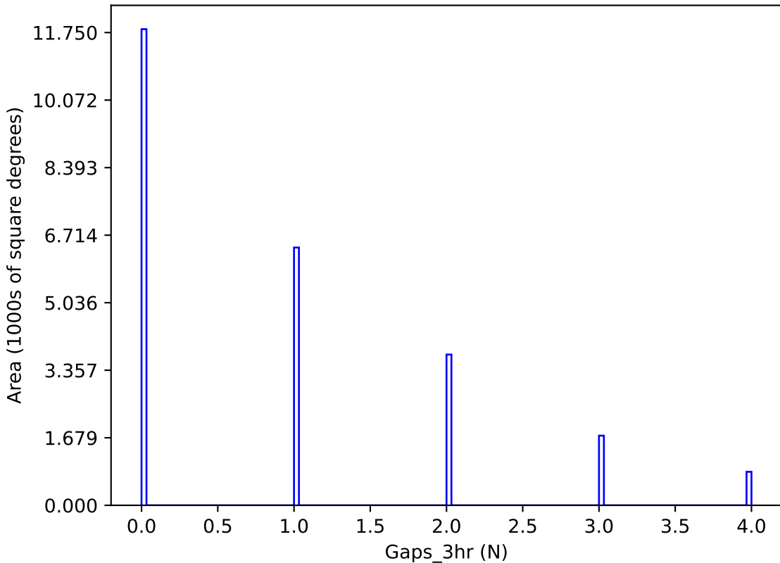
early_u_fpextra2.0_v3.4_10yrs y band: Gaps_3hr
