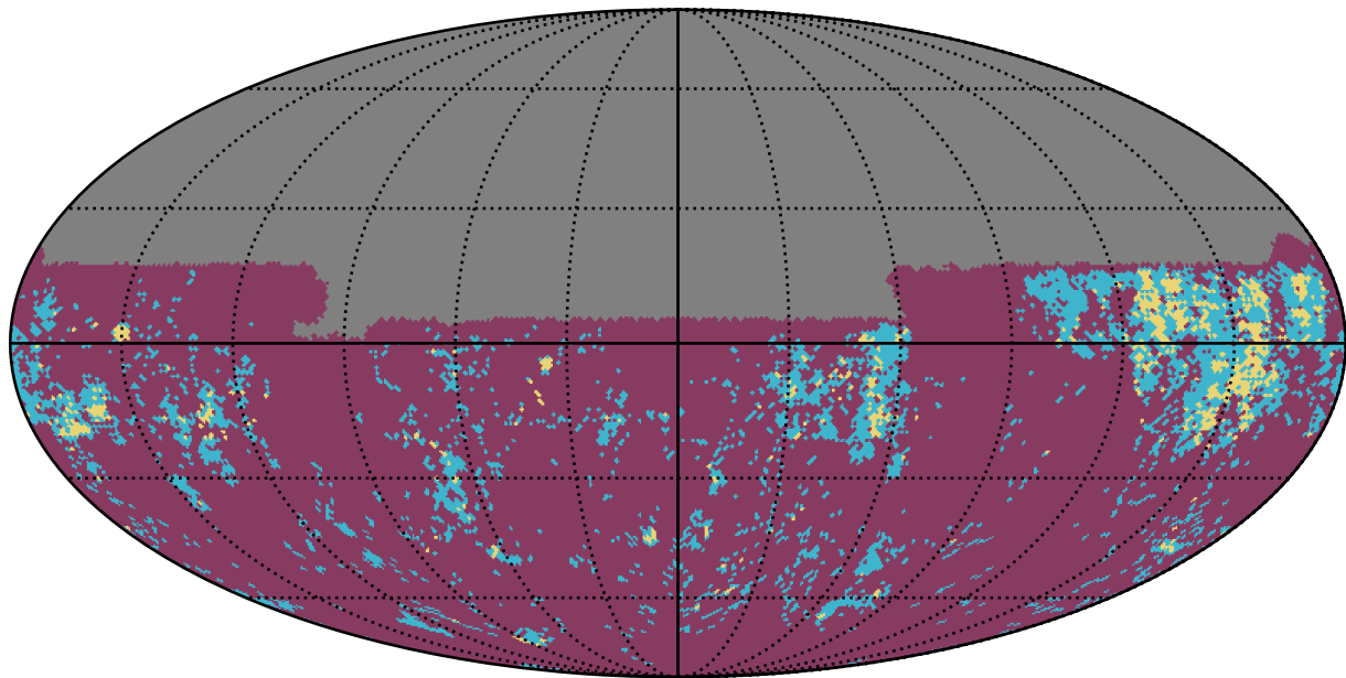
early_u_fpextra2.0_v3.4_10yrs u band: Gaps_3hr
