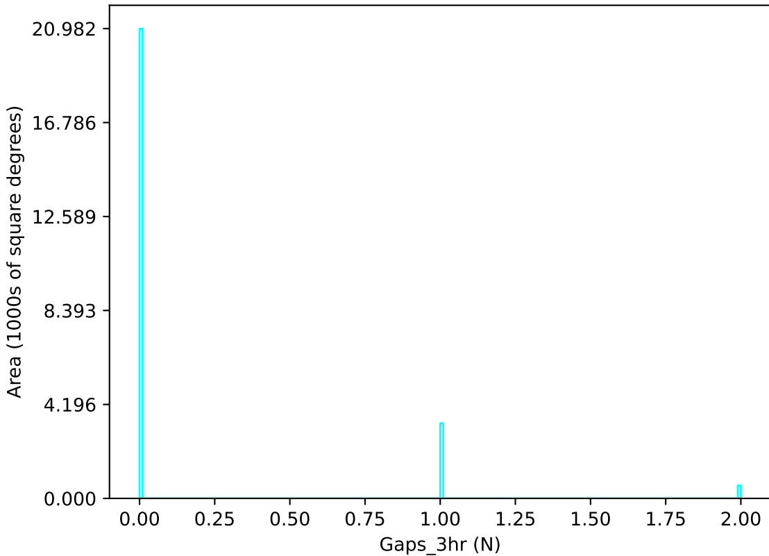
early_u_fpextra2.0_v3.4_10yrs u band: Gaps_3hr
