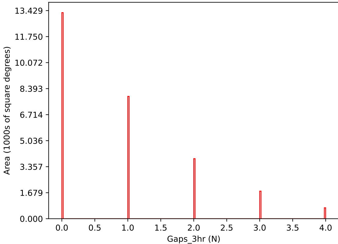
early_u_fpextra2.0_v3.4_10yrs i band: Gaps_3hr
