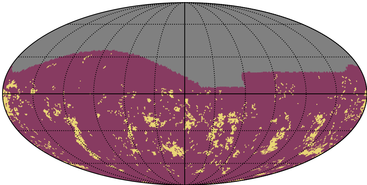
early_u_fpextra2.0_v3.4_10yrs g band: Gaps_3hr
