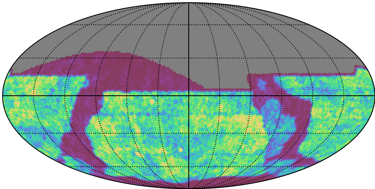
early_u_fpextra2.0_v3.4_10yrs z band: Gaps_24hr
