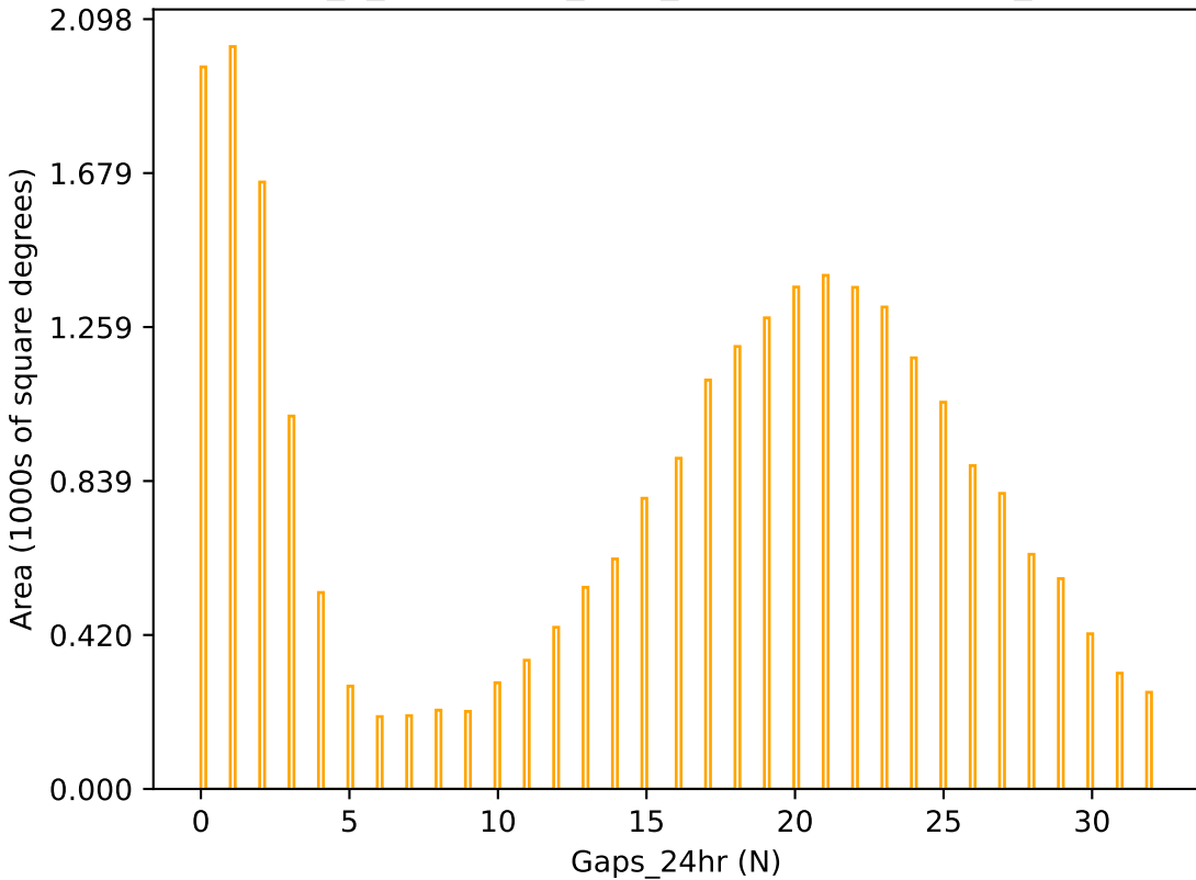
early_u_fpextra2.0_v3.4_10yrs r band: Gaps_24hr
