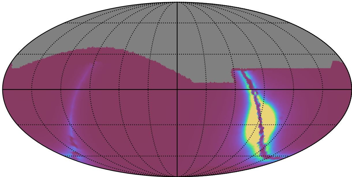
early_u_fpextra2.0_v3.4_10yrs : GalplaneFootprintMetric_xray_binaries_map_Tau_46_5
