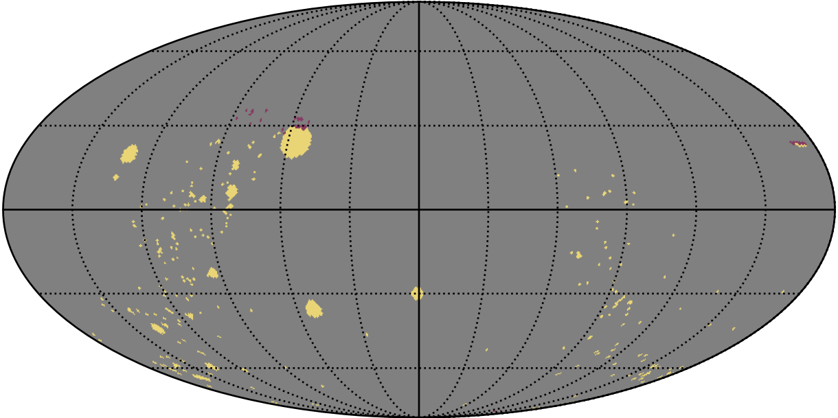
early_u_fpextra2.0_v3.4_10yrs : GalplaneFootprintMetric_open_clusters_map_Tau_73_0
