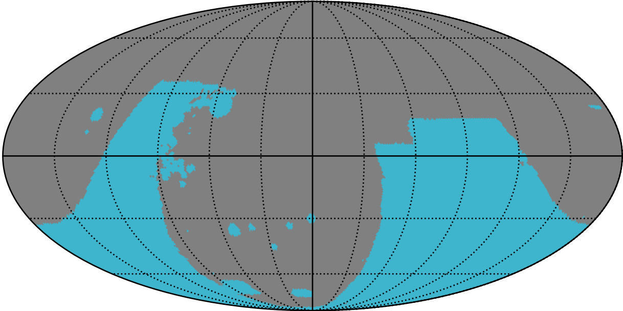
early_u_fpextra2.0_v3.4_10yrs : GalplaneFootprintMetric_combined_map_Tau_2_0
