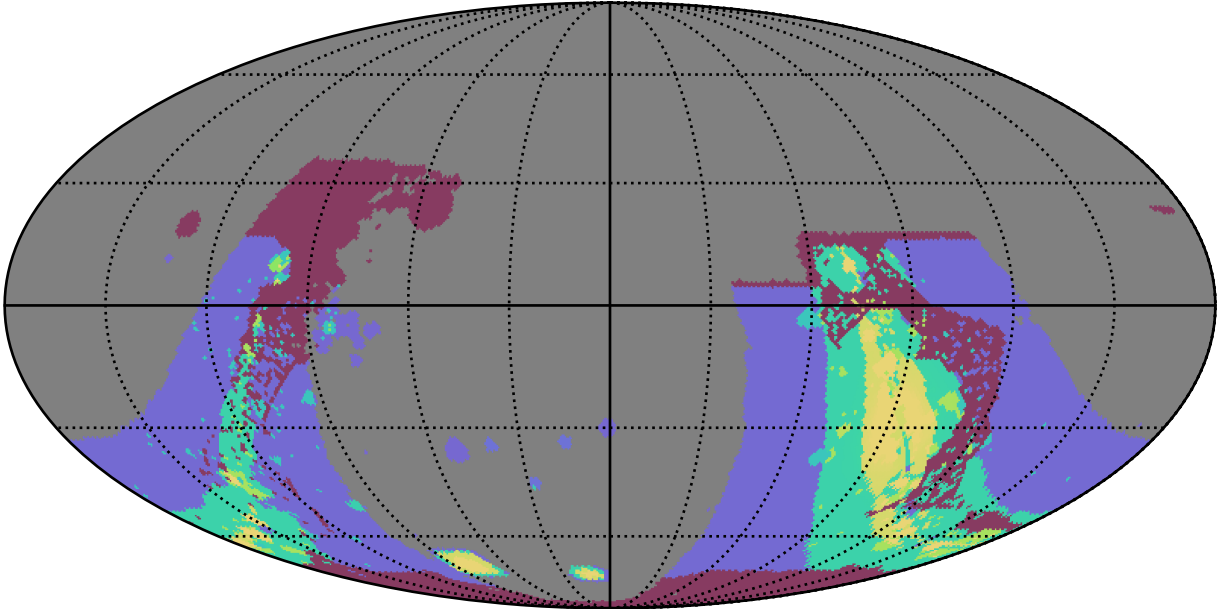
early_u_fpextra2.0_v3.4_10yrs : GalplaneFootprintMetric_combined_map_Tau_20_0
