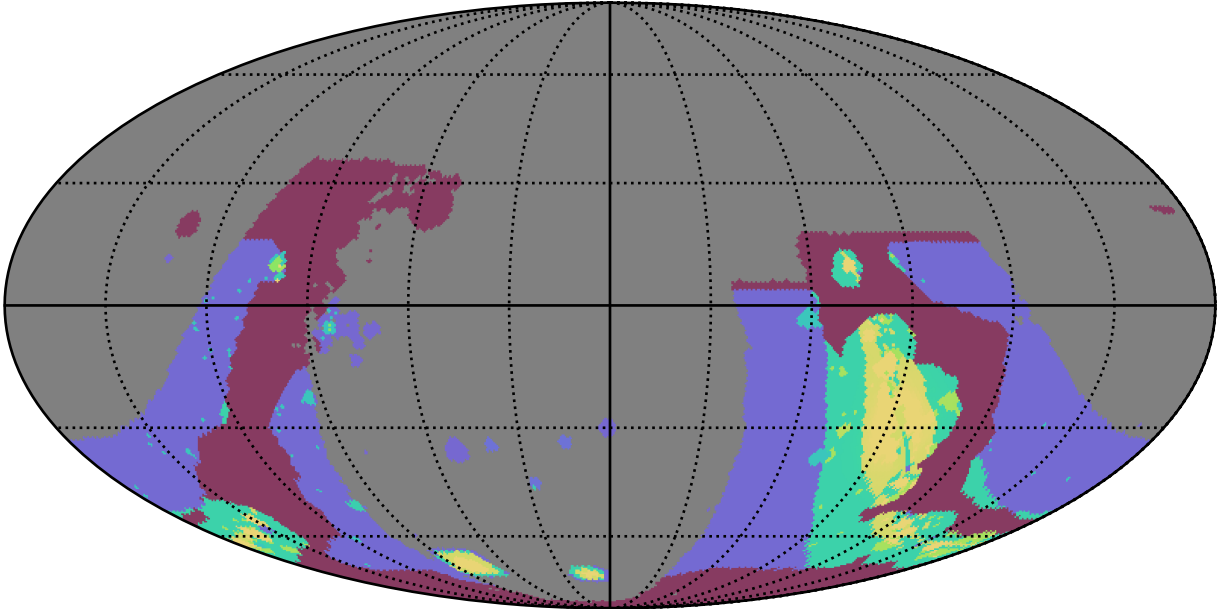
early_u_fpextra2.0_v3.4_10yrs : GalplaneFootprintMetric_combined_map_Tau_11_0
