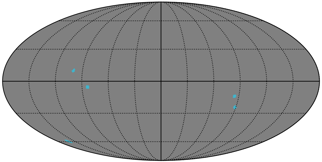
early_u_fpextra2.0_v3.4_10yrs : GalplaneFootprintMetric_bonito_sfr_map_Tau_5_0
