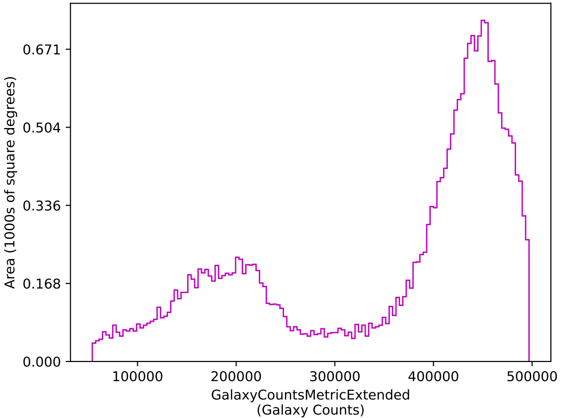
early_u_fpextra2.0_v3.4_10yrs z: GalaxyCountsMetricExtended
