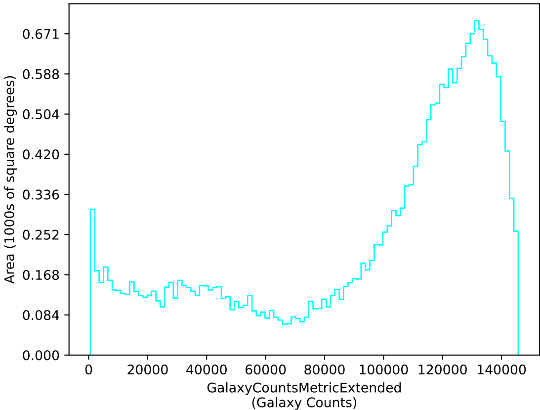
early_u_fpextra2.0_v3.4_10yrs u: GalaxyCountsMetricExtended
