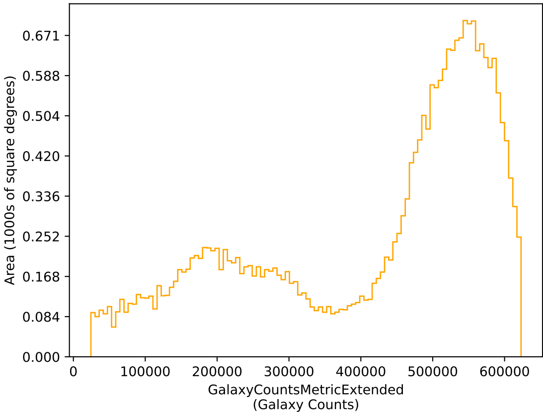
early_u_fpextra2.0_v3.4_10yrs r: GalaxyCountsMetricExtended
