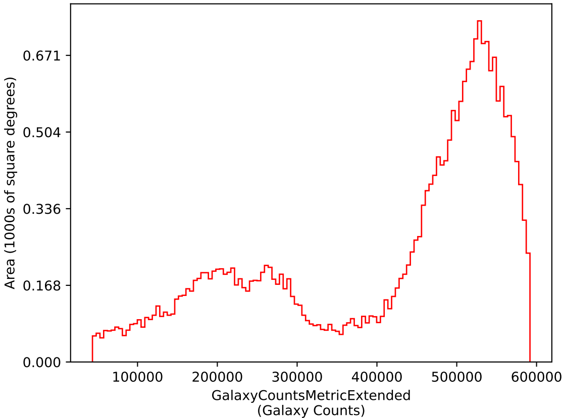
early_u_fpextra2.0_v3.4_10yrs i: GalaxyCountsMetricExtended
