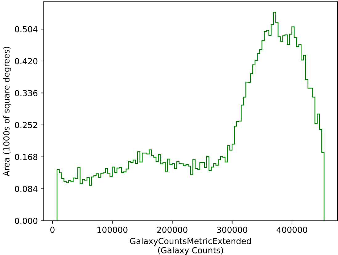
early_u_fpextra2.0_v3.4_10yrs g: GalaxyCountsMetricExtended
