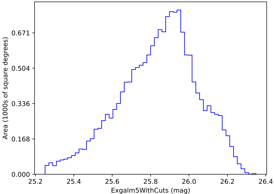
early_u_fpextra2.0_v3.4_10yrs i band non-DD year 3: ExgalM5WithCuts
