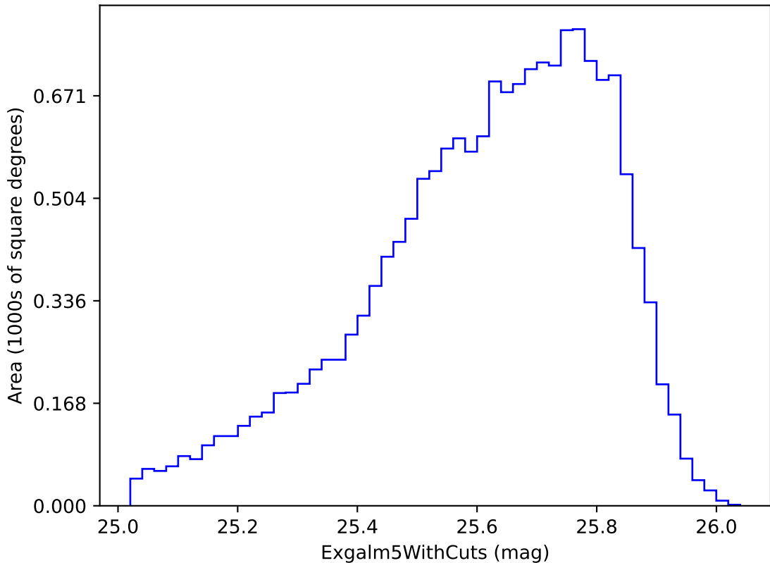
early_u_fpextra2.0_v3.4_10yrs i band non-DD year 2: ExgalM5WithCuts
