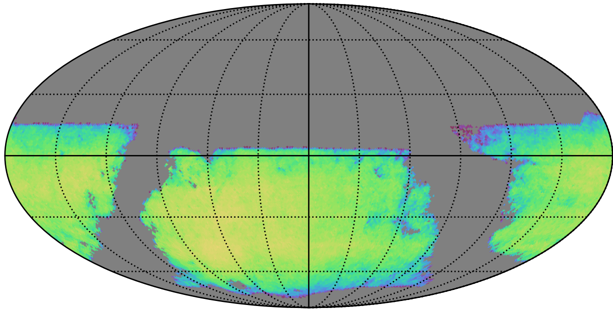
early_u_fpextra2.0_v3.4_10yrs i band galaxies non-DD: DepthLimitedNumGalaxiesMetric
