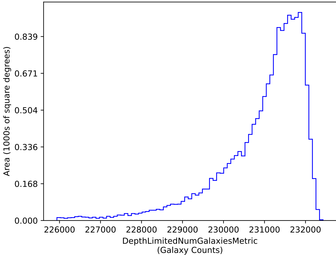
early_u_fpextra2.0_v3.4_10yrs i band galaxies non-DD: DepthLimitedNumGalaxiesMetric
