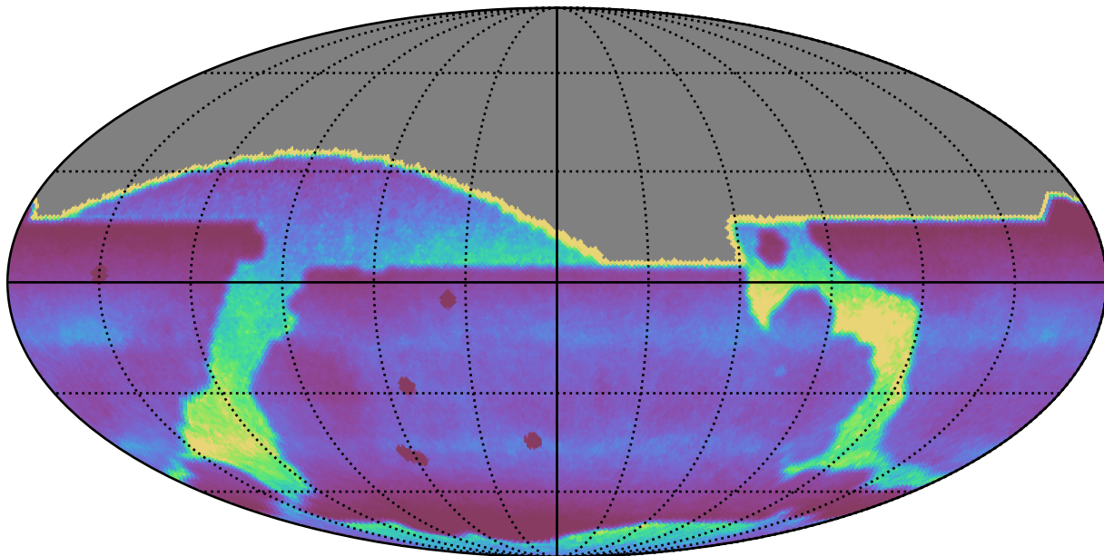
early_u_fpextra2.0_v3.4_10yrs : DCRprecision
