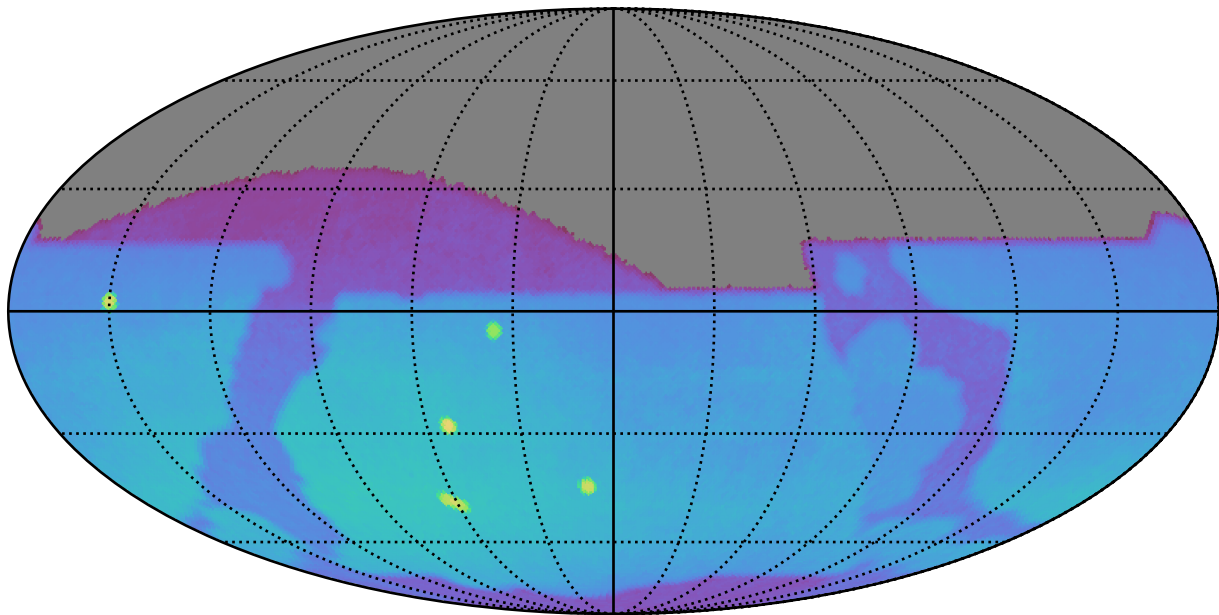
early_u_fpextra2.0_v3.4_10yrs : Brown Dwarf, L7
