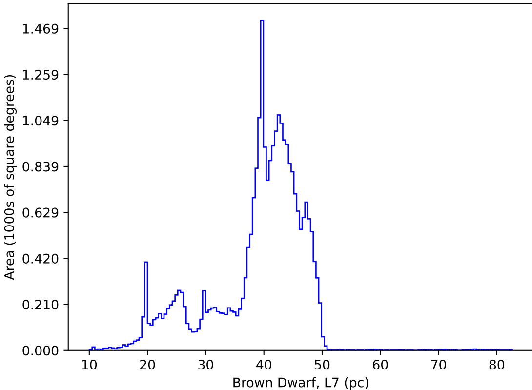
early_u_fpextra2.0_v3.4_10yrs : Brown Dwarf, L7
