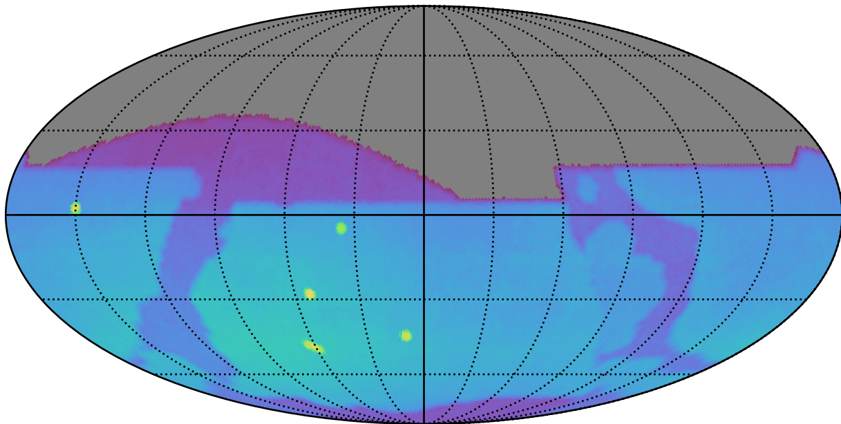
early_u_fpextra2.0_v3.4_10yrs : Brown Dwarf, L4
