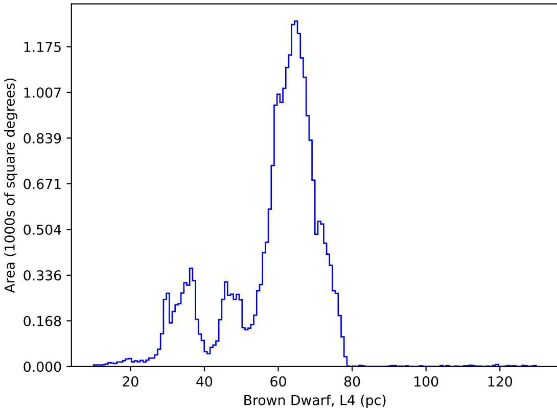
early_u_fpextra2.0_v3.4_10yrs : Brown Dwarf, L4
